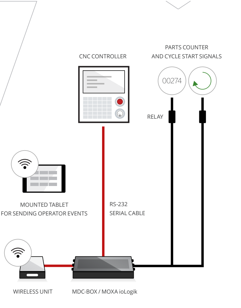
EXAMPLE OF WIRELESS NETWORK WITH HARDWARE CONNECTION USING MDC-BOX / MOXA ioLogik
