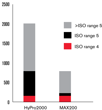
Cut quality over life (200 A) 12 mm (1/2") mild steel, 15 m (50') leads
